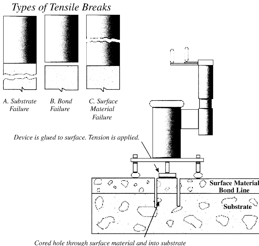
Fig. 5—Test procedure.
