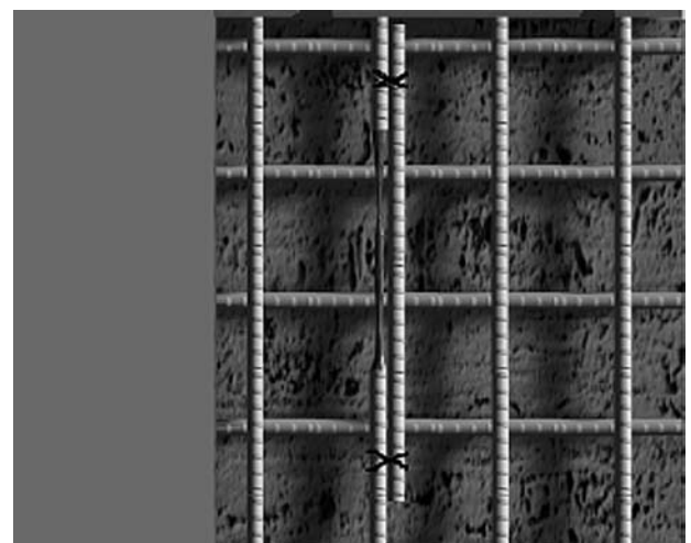
Fig. 2—Lapping of supplemental reinforcing.
