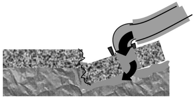
Fig. 5—Pumping of the slabjacking grout in the drilled hole showing grout flow resulting in slab displacement.
