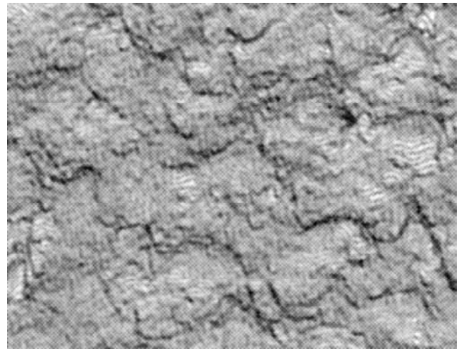
Fig. 1—Typical plus or minus 1/4 in. profile. (From ICRI Guide No. 03732 Profile No. 7). This is the standard recommended surface profile for low-pressure spray-applied mortars.
